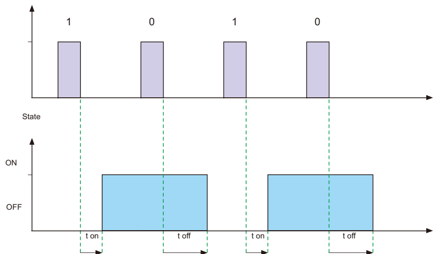
KNX telegram
