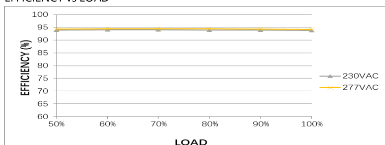
EFFICIENCY vs LOAD
