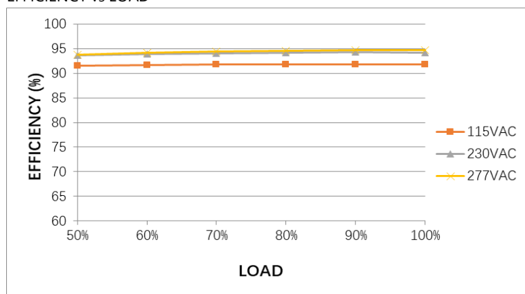
EFFICIENCY vs LOAD
