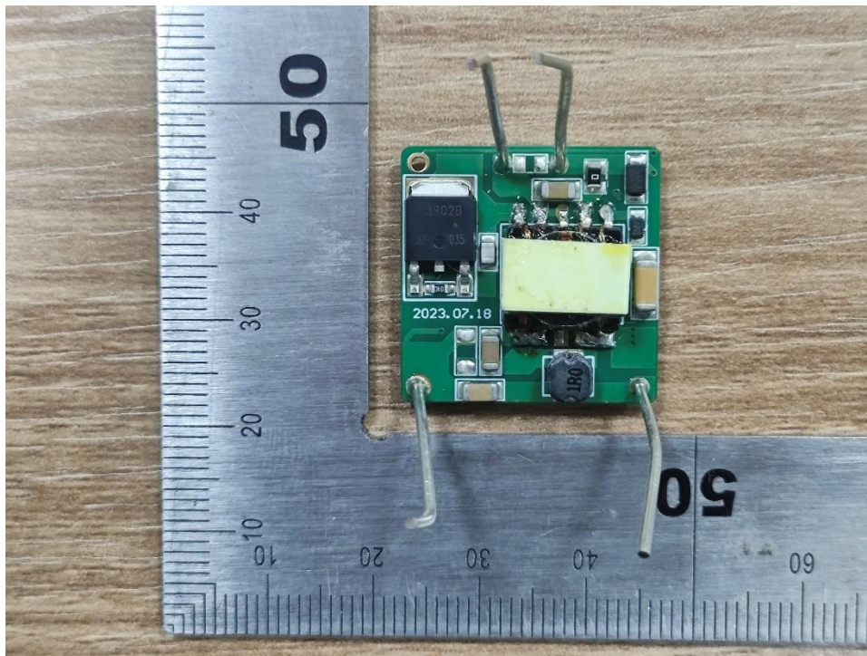
Bild / Picture 6: Power board view
