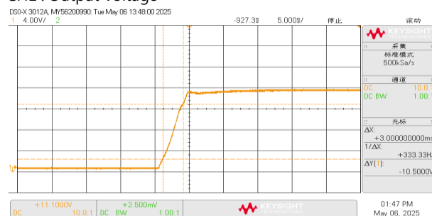
INPUT=115VAC/60HZ @ FULL LOAD CH1 : Output Voltage
