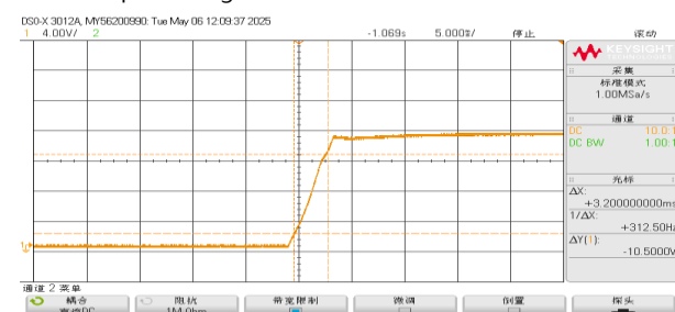
INPUT=230VAC/50HZ @ FULL LOAD CH1 : Output Voltage
