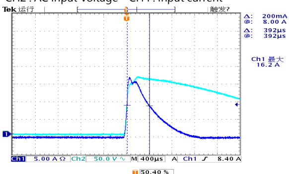
INPUT=115VAC/50HZ @ FULL LOAD
