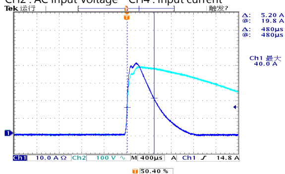
INPUT=115VAC/50HZ @ FULL LOAD
