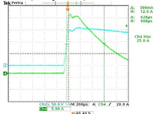
INPUT=115VAC/ 60HZ @ FULL LOAD
